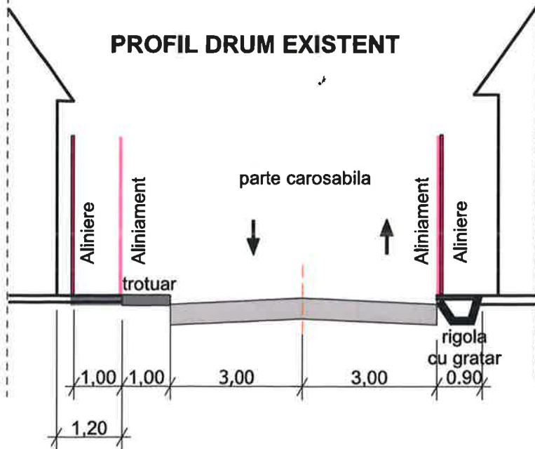
PROFIL DRUM PROPUȘ
